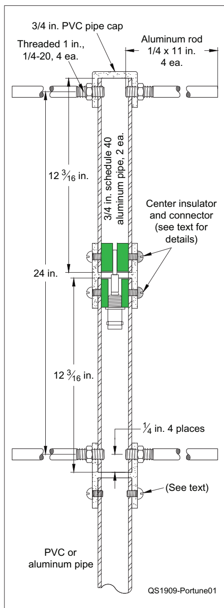
Figure 1 — Mechanical drawing of the rugged 2-meter antenna.
