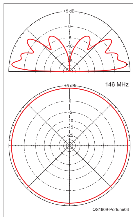
Figure 3 — Elevation and azimuth radiation patterns.
