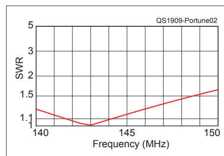
Figure 2 — SWR sweep from 140 MHz to 150 MHz.
