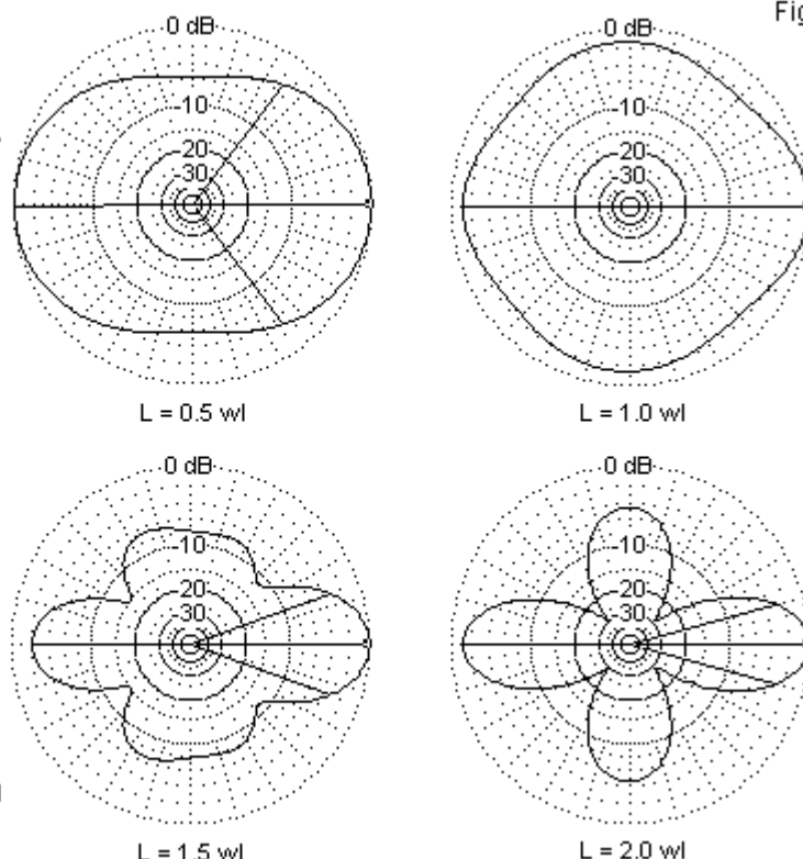
Quadrant Antenna Azimuth Patterns at Various Lengths Relative to the Operating Frequency
