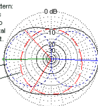
L-Antenna at 1 Wavelength above Average Ground Azimuth and Elevation Patterns with Vertical and Horizontal Components
